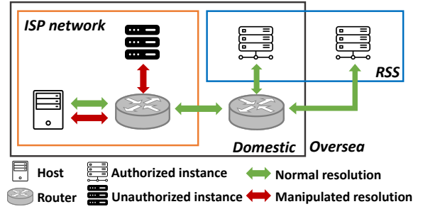
Fig. 1. Threat model of unauthorized instances.
