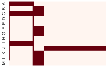
Fig. 9. The vantage points cannot access root servers. A red cell indicates that the root server (X-axis) was unavailable to the vantage point (Y-axis).
